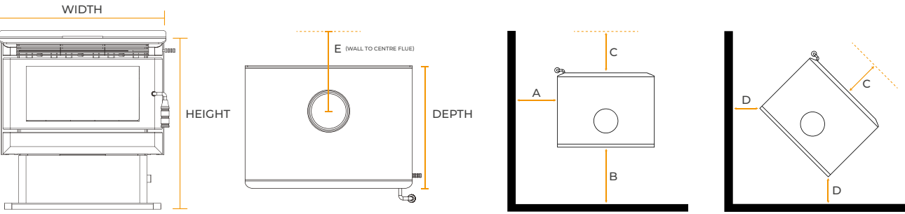
Unit Size and Clearances (mm)
