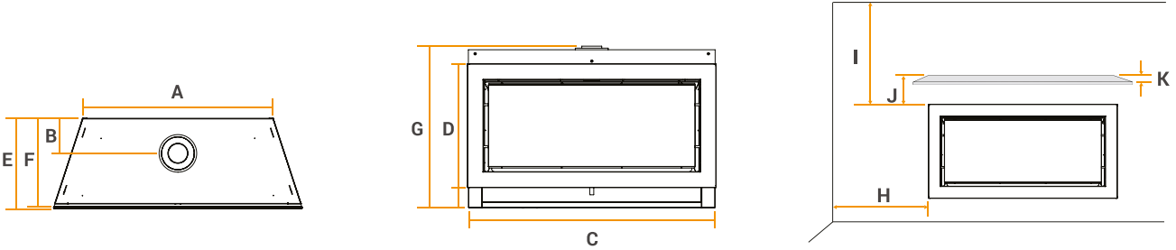
Unit Size and Clearances (mm)
